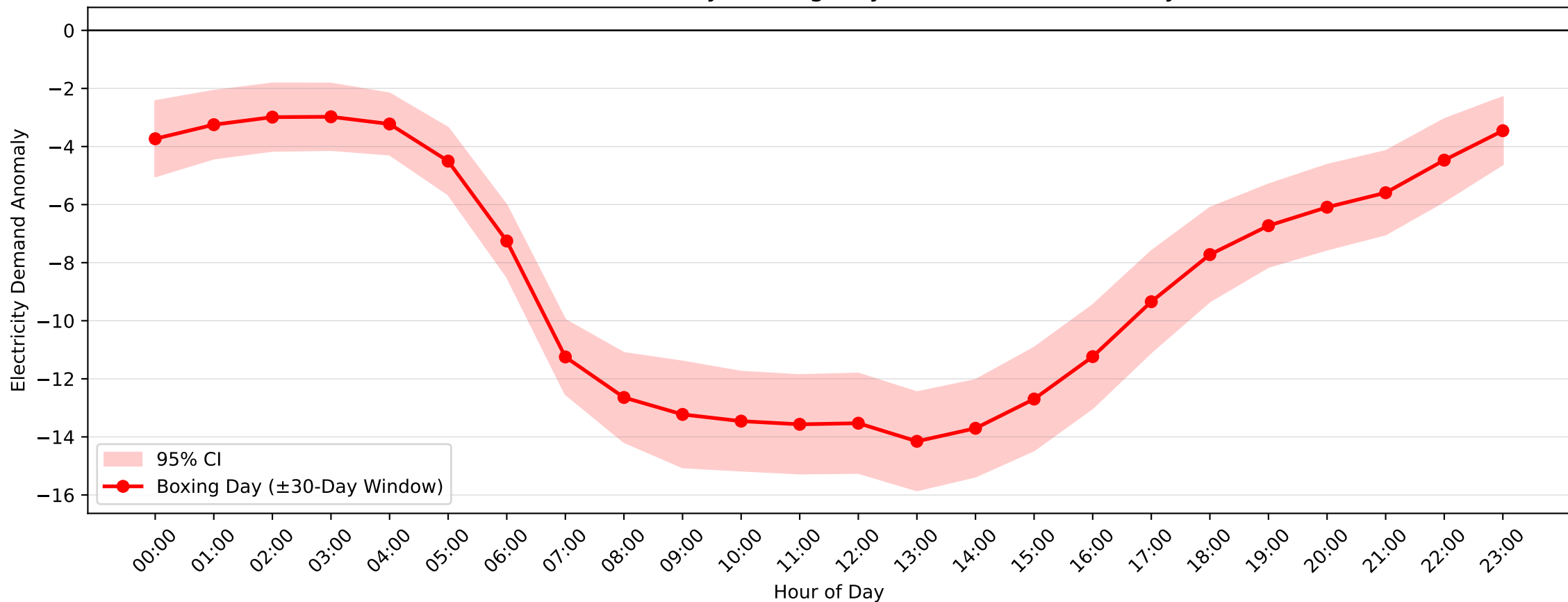
St. Peters Demand Anomaly: Boxing Day (2004–2017, \pm 30 -Day Window)
